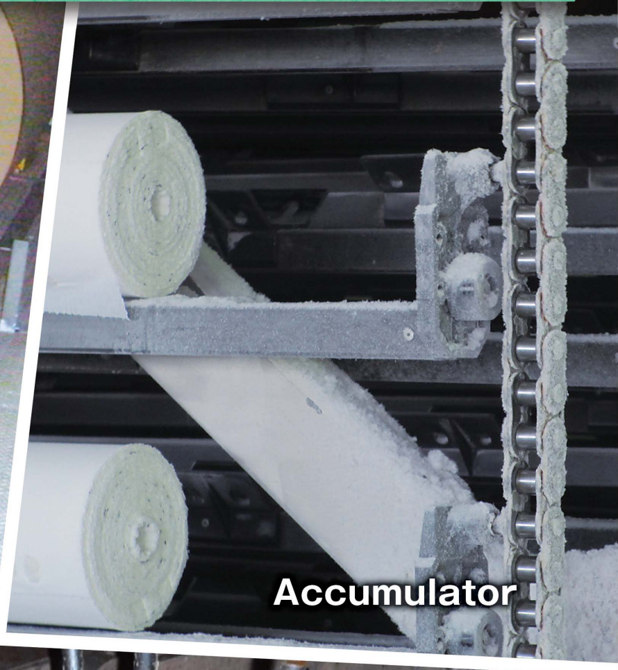
Web Conveyance
