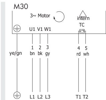
Fig.: 3-phase, 4+2 core cable, winding for 1 voltage, delta connection
