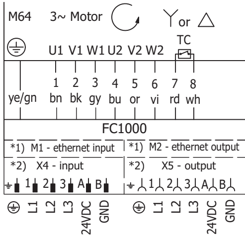
Fig.: 3-phase, 7-core cable, winding for 2 voltages, delta or star connection
