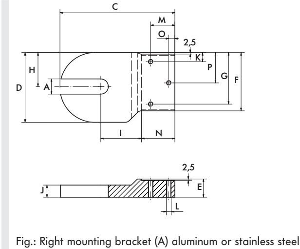
DM 0113, DM 0138 and DM 0165 dimensions
