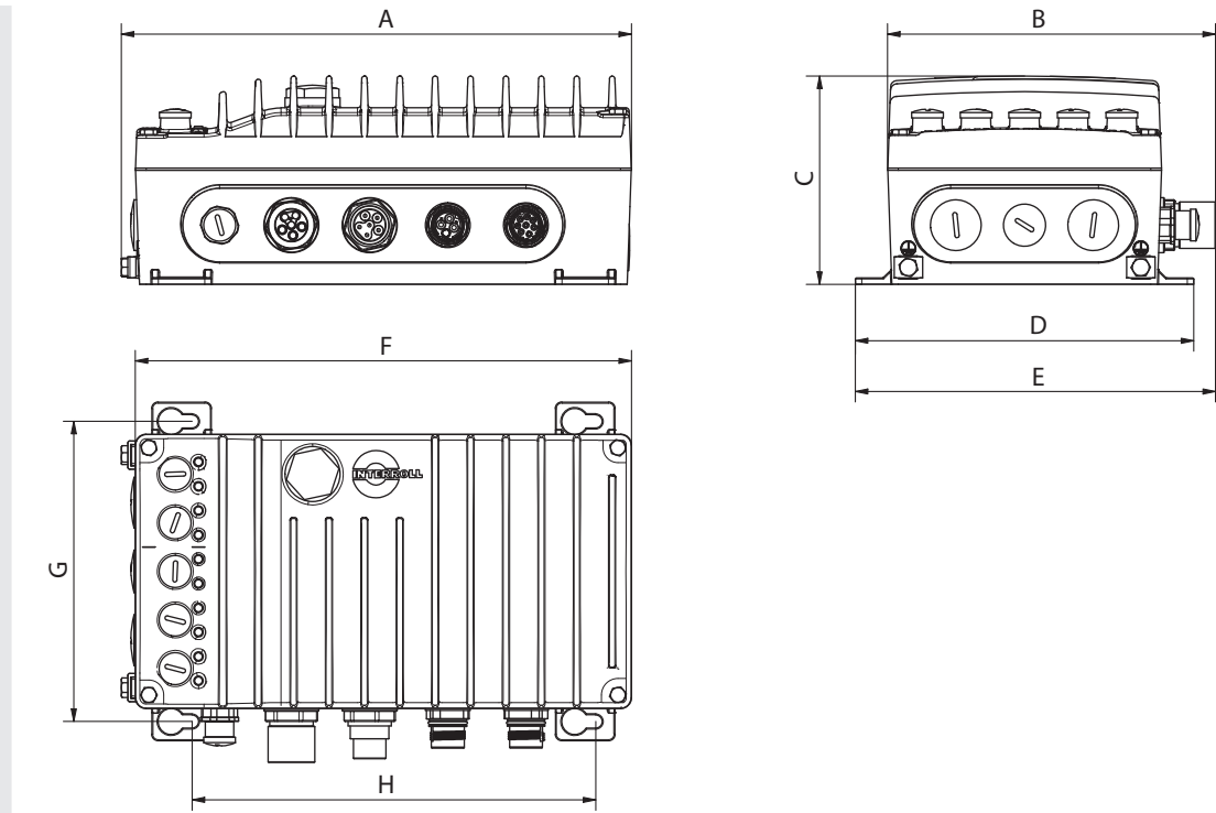
Fig.: FC 1000, wall-mounted, size 1, 2 & 3
