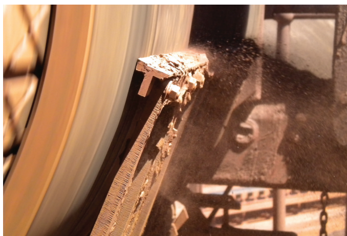
Shown: H-Type® V-Tip Precleaner
