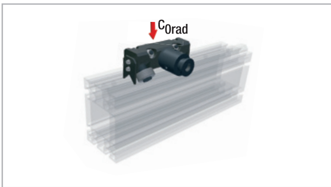
Important: remove the space washers to enable self-alignment of the roller slide Fig. 18
