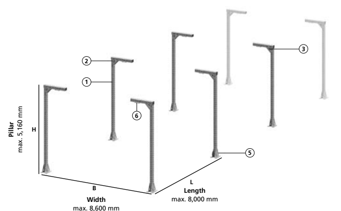
Modular cantilever arm KBG-C Maximum lift capacity 85 kg
