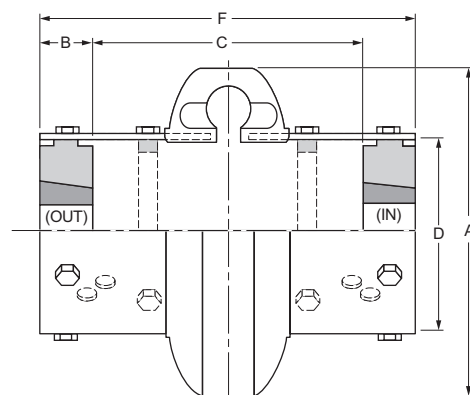
Taper-Lock
