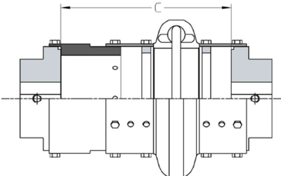
SINGLE EXTENSION
