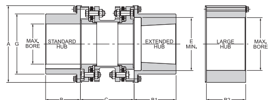
8-Bolt Design
