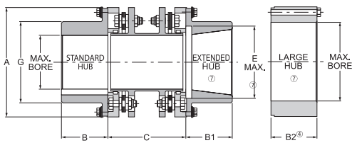
4- & 6-Bolt Design
