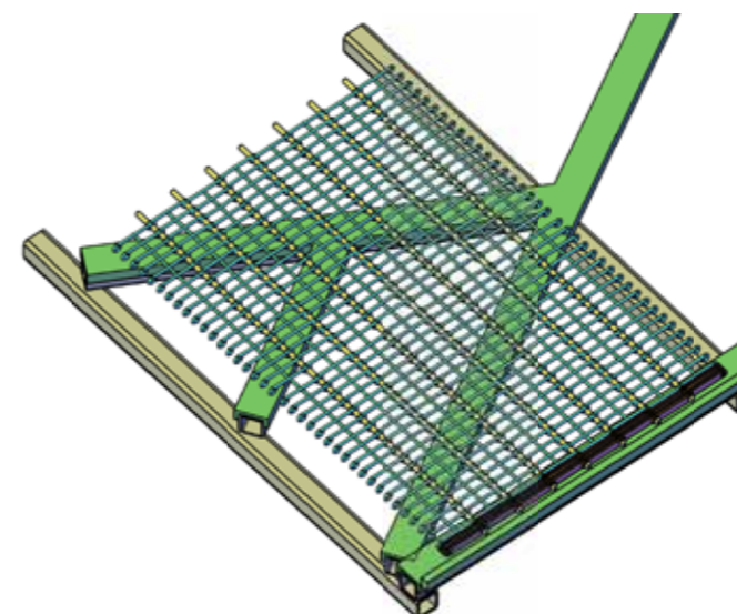
Herringbone support
