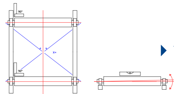
Geometry of the frame
