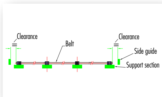
Side guidance
