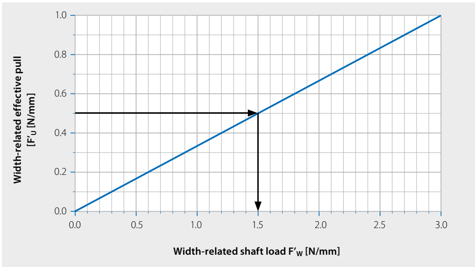
Diagram 1: Identifying the minimum shaft load
