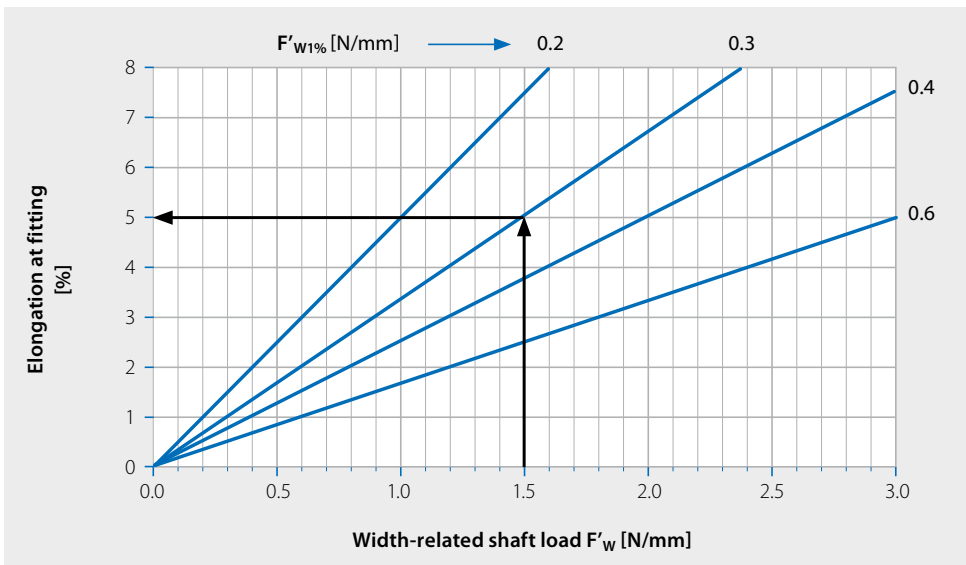
Diagram 2: Identifying the elongation at fitting
