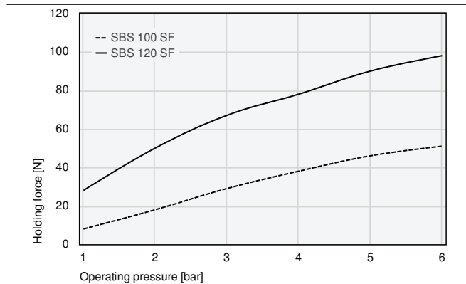
Holding force
