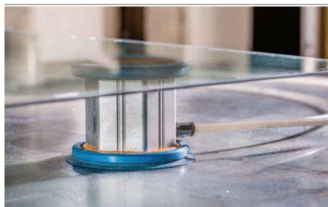
Vacuum block VCBL-GL clamping glass
