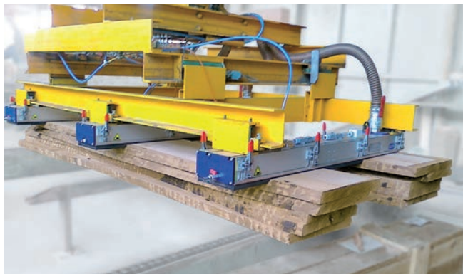
Area Gripping System SBX-C on an portal when handling wooden boards
