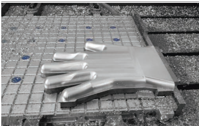
Matrix plate for clamping aluminum parts
