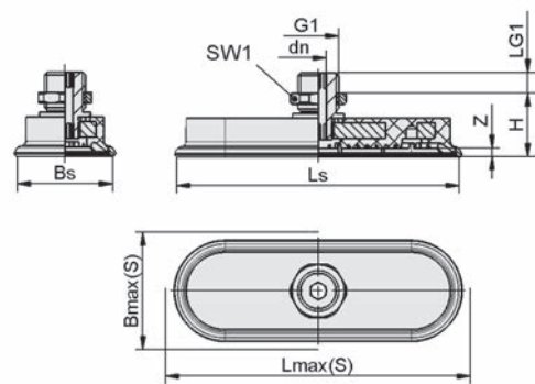
SAOF HT2 AG
