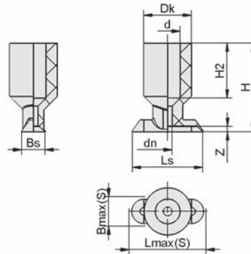
SGON 15x5 - 90x30 IG
