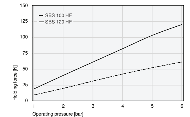
Holding force
