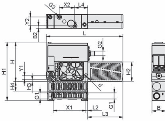
SX(M)Pi H
