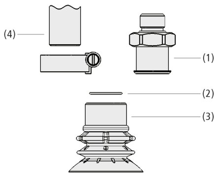
System Design Bellows Suction Cups SPB2f (2.5 Folds)
